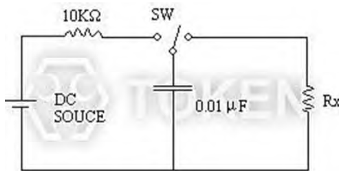
Test Circuit
