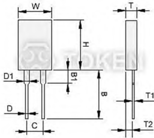
TO220 Power Resistors (RMG20) Dimensions (Unit: mm)
