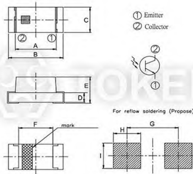
SMD Light Sensor (PT-B1-DC-0603-940) Dimensions
