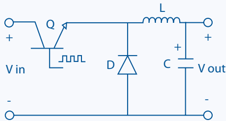
Simplified Buck Regulator
