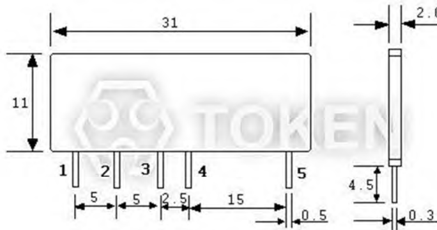
High Voltage Divider Network (NTK-A) Series Dimensions
