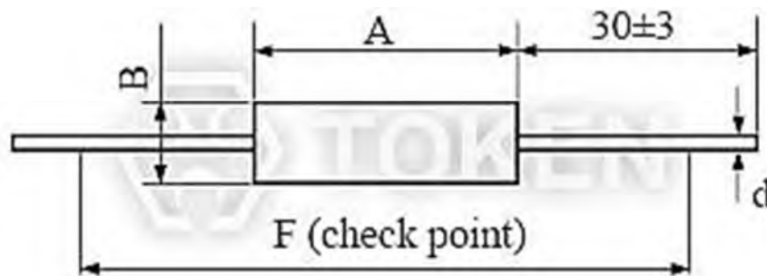
Precision Wire wound (BWW) Dimensions
