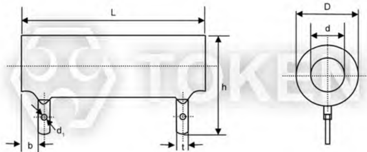
Power Wirewound Glaze Resistors (DRB20) Dimensions (Unit: mm)
