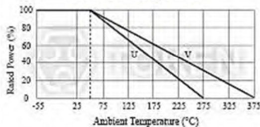
Power Derating Curve
