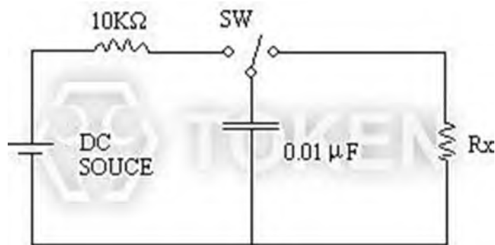
Test Circuit
