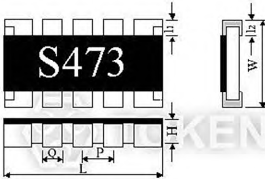
Resistor Chip Networks (RCN) Dimensions
