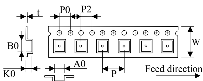
2. Tape Dimensions
